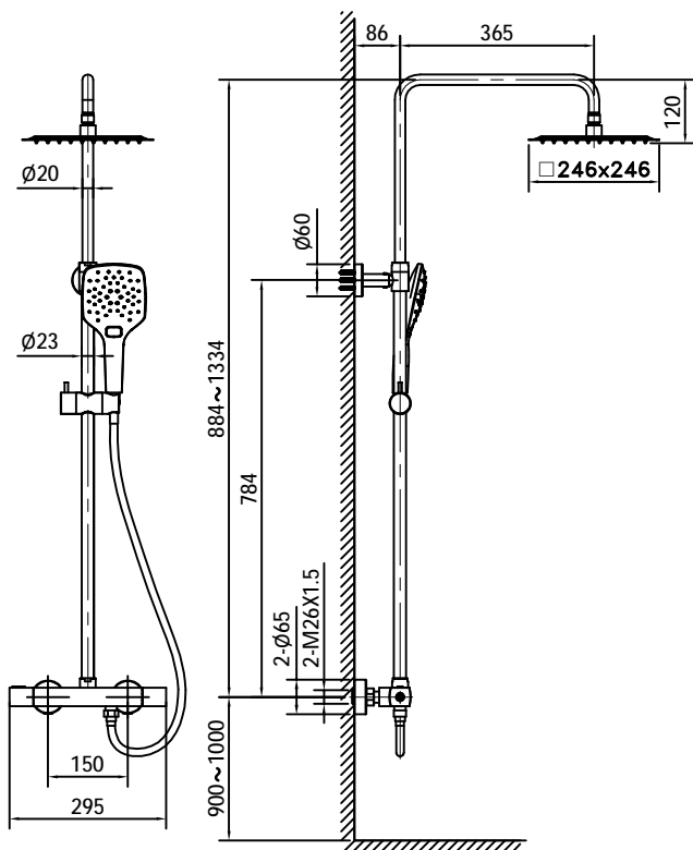
Installation drawing
