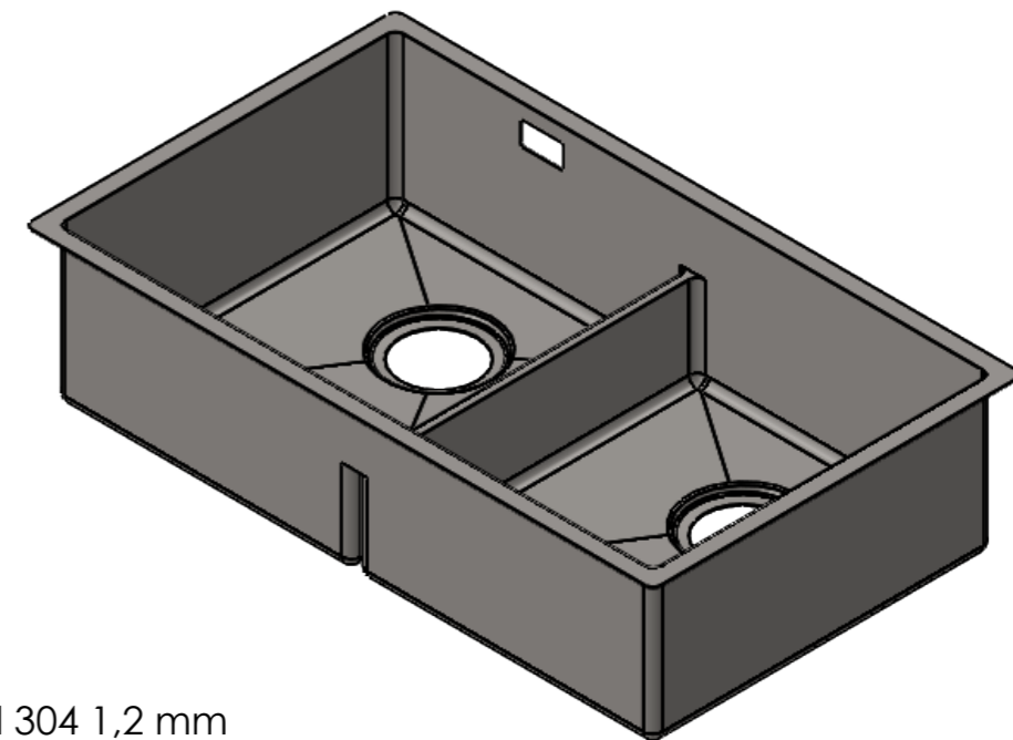
DETAIL B
