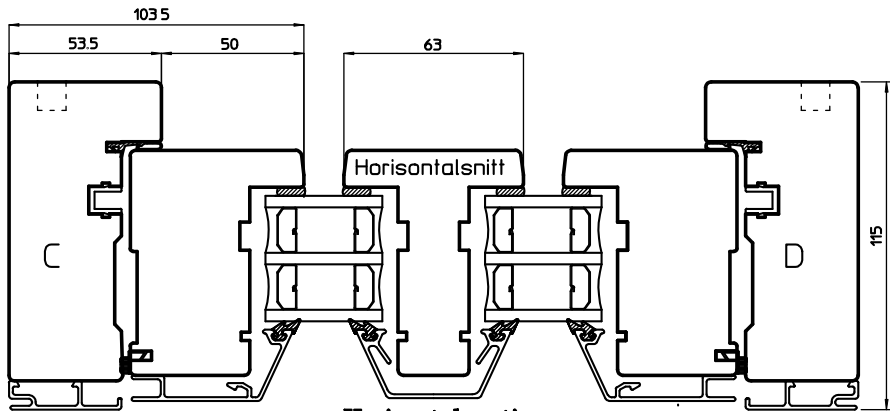
Horizontal section
